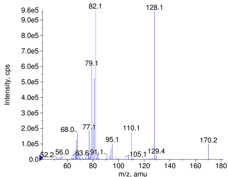
+ Aceclidine Prec(170.0) CE(50.0) RT(0.8)
