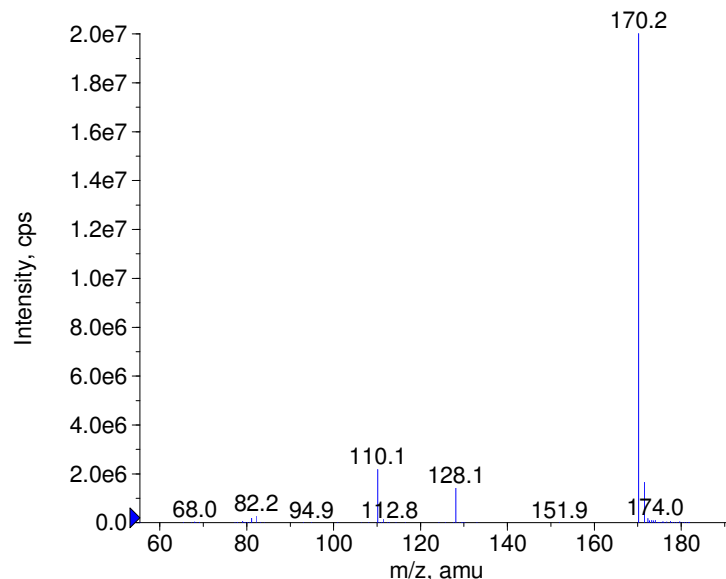
+ Aceclidine Prec(170.0) CE(50.0) RT(0.8)
