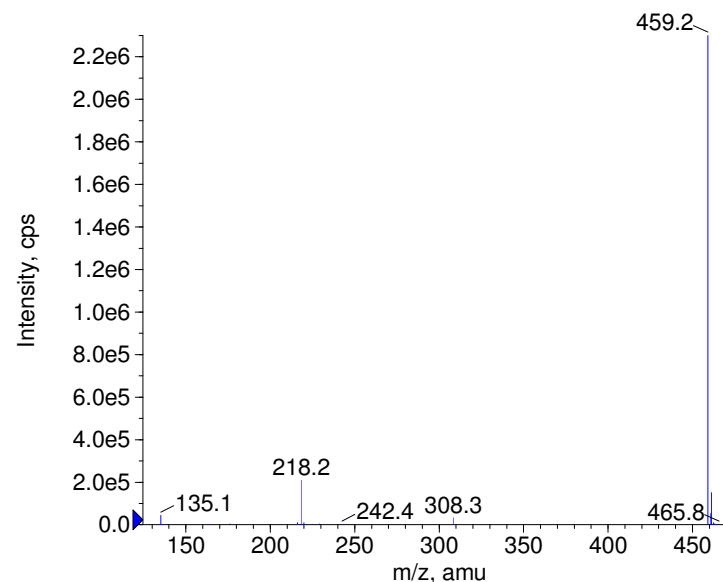
+ Astemizole Prec(459.0) CE(50.0) RT(0.8)
