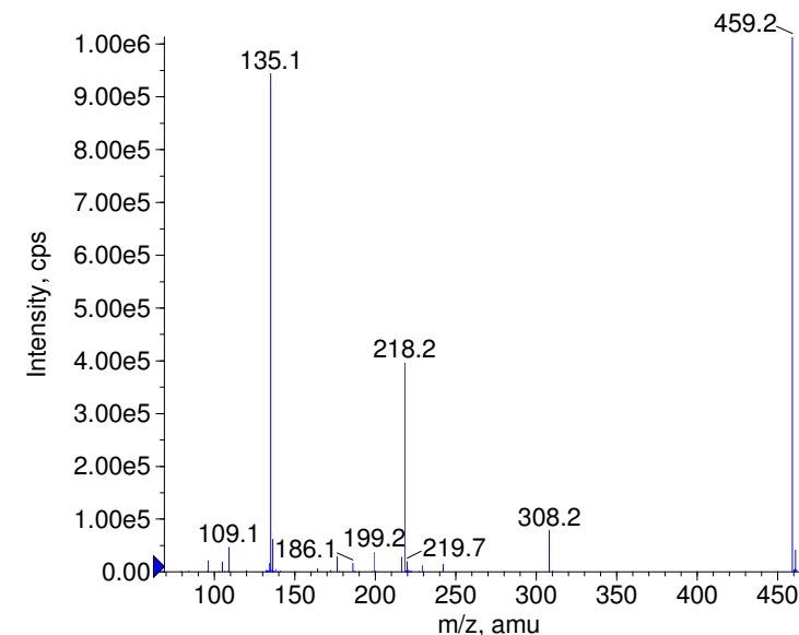
+ Astemizole Prec(459.0) CE(99.0) RT(0.8)
