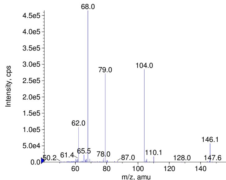
+ Atrazine-desethyl Prec(188.0) CE(50.0) RT(1.0)
