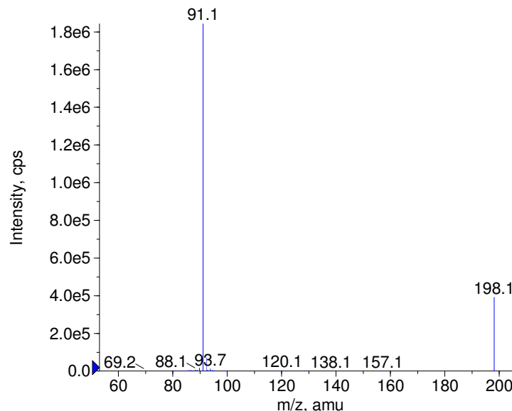
+ Beclamide Prec(198.0) CE(50.0) RT(1.2)
