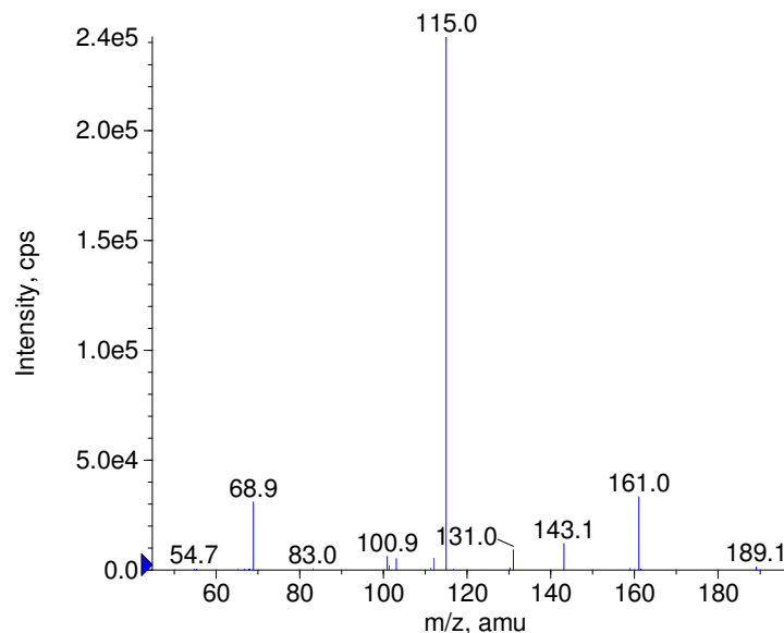
■ - Benzyltetric acid Prec(189.0) CE(-50.0) RT(0.8)
