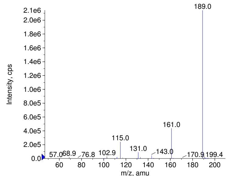
■ - Benzyltetric acid Prec(189.0) CE(-99.0) RT(0.8)
