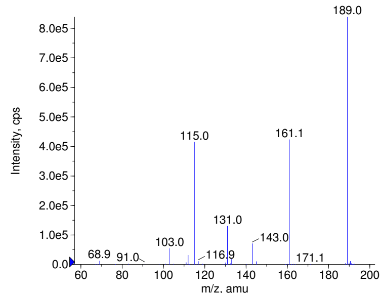
■ - Benzyltetric acid Prec(189.0) CE(-99.0) RT(0.8)
