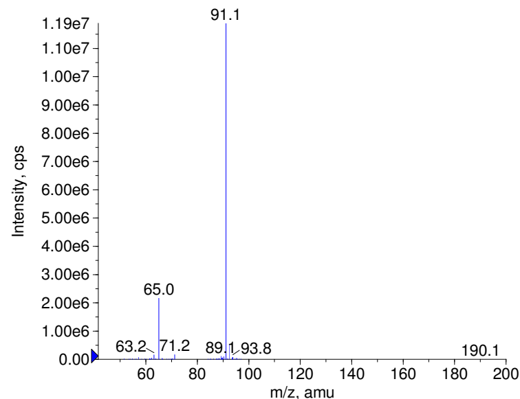
+ Bethanidine Prec(178.0) CE(50.0) RT(0.9)
