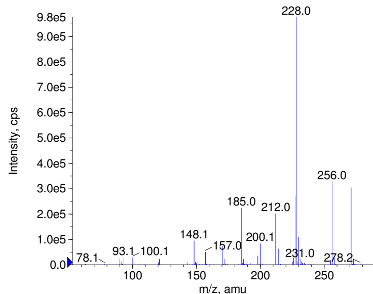
+ Bromopride Prec(344.0) CE(50.0) RT(0.9)
