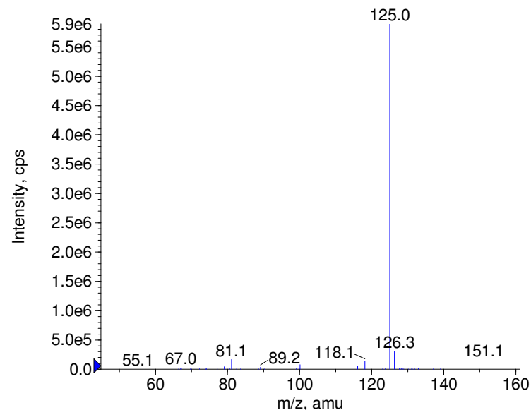
+ Chlorphencyclan Prec(310.0) CE(50.0) RT(0.9)
