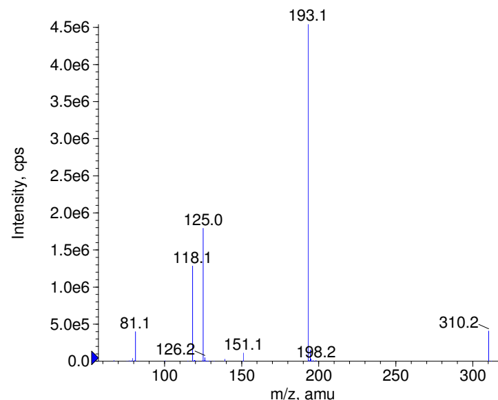
+ Chlorphencyclan Prec(310.0) CE(50.0) RT(0.9)
