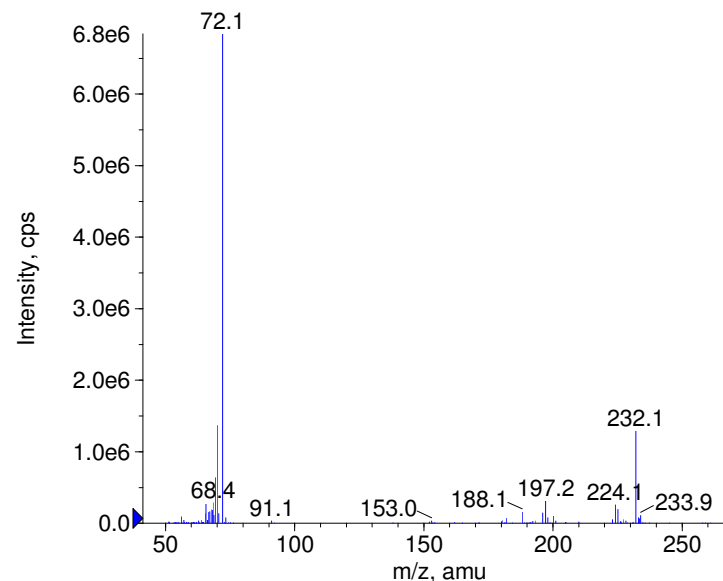
+ Chlorphenethiazine Prec(305.0) CE(50.0) RT(0.9)
