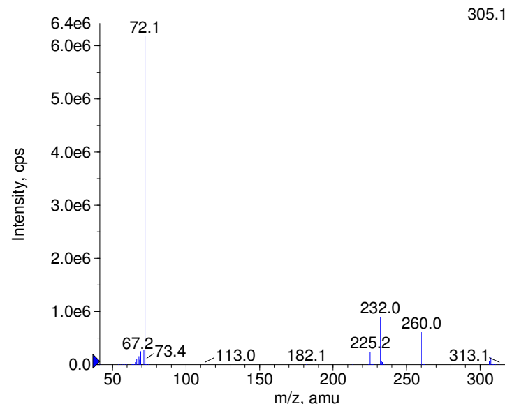
+ Chlorphenethiazine Prec(305.0) CE(50.0) RT(0.9)
