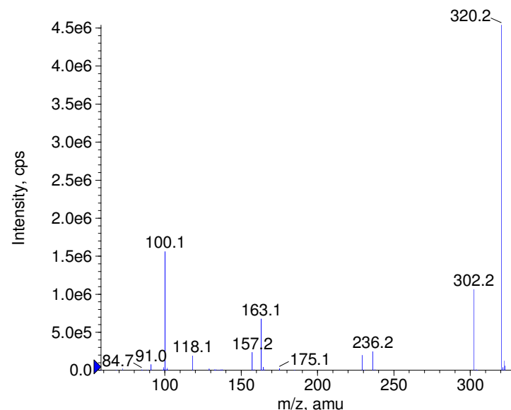
+ Cyclodrine Prec(320.0) CE(50.0) RT(0.9)
