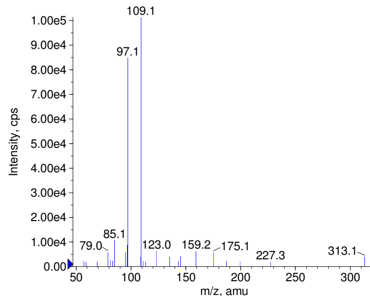
+ Desoxycortone enantate Prec(443.0) CE(50.0) RT(5.5)
