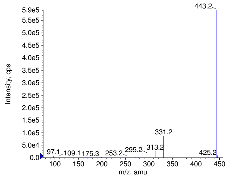
+ Desoxycortone enantate Prec(443.0) CE(50.0) RT(5.5)
