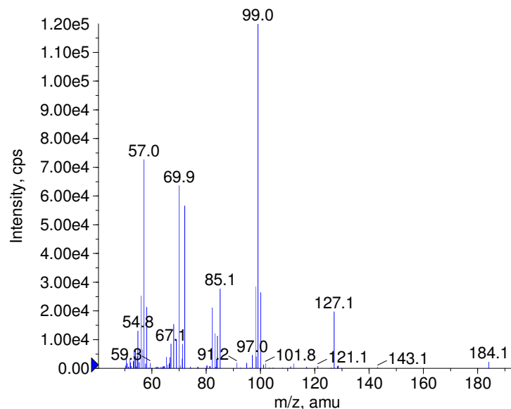
+ Diethylcarbamazine Prec(200.0) CE(50.0) RT(0.7)
