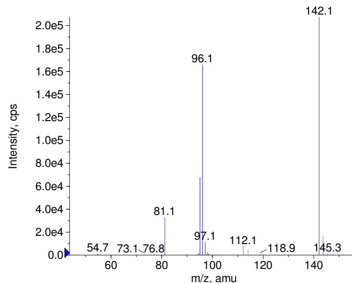
+ Dimetridazole Prec(142.0) CE(50.0) RT(0.9)
