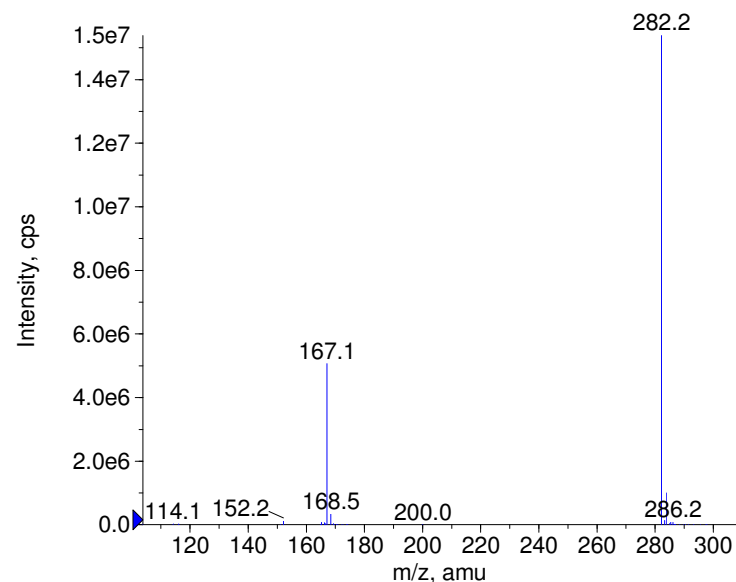
+ Diphenylpyraline Prec(282.0) CE(50.0) RT(0.9)
