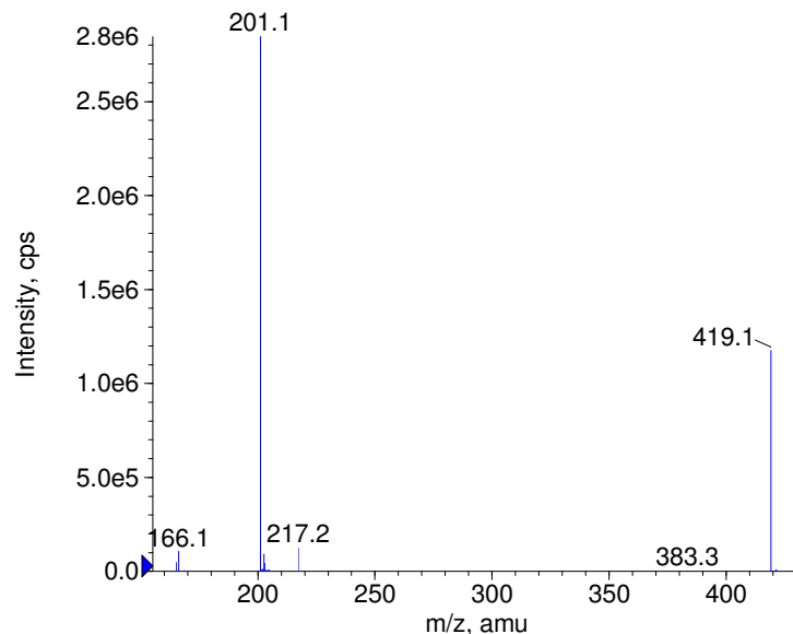
+ Etodroxizine Prec(419.0) CE(50.0) RT(1.1)
