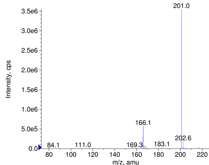
+ Etodroxizine Prec(419.0) CE(99.0) RT(1.1)
