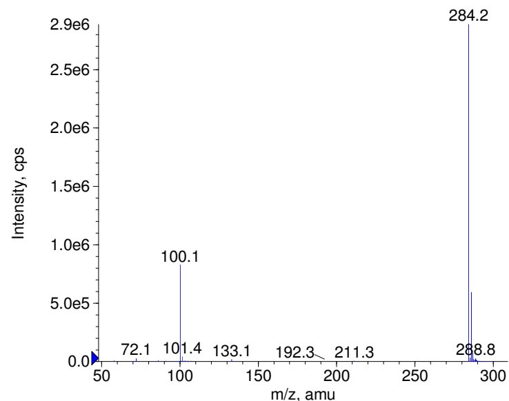
+ Etoloxamine Prec(284.0) CE(50.0) RT(0.9)
