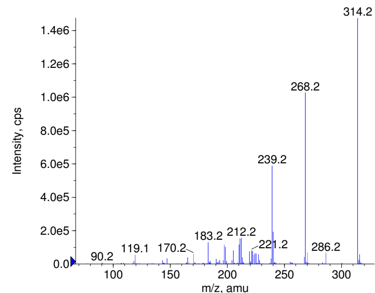
+ Flunitrazepam Prec(314.0) CE(99.0) RT(0.8)
