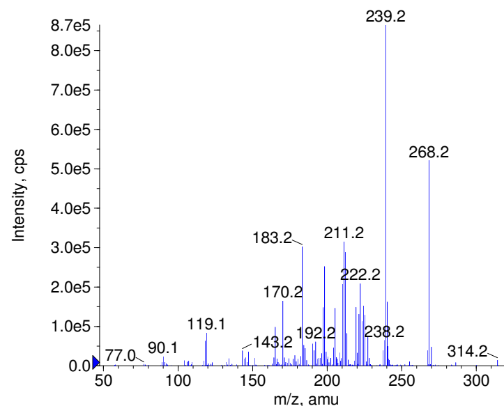
+ Flunitrazepam Prec(314.0) CE(50.0) RT(0.8)
