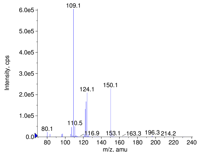
+ Flupirtine Prec(305.0) CE(50.0) RT(0.8)
