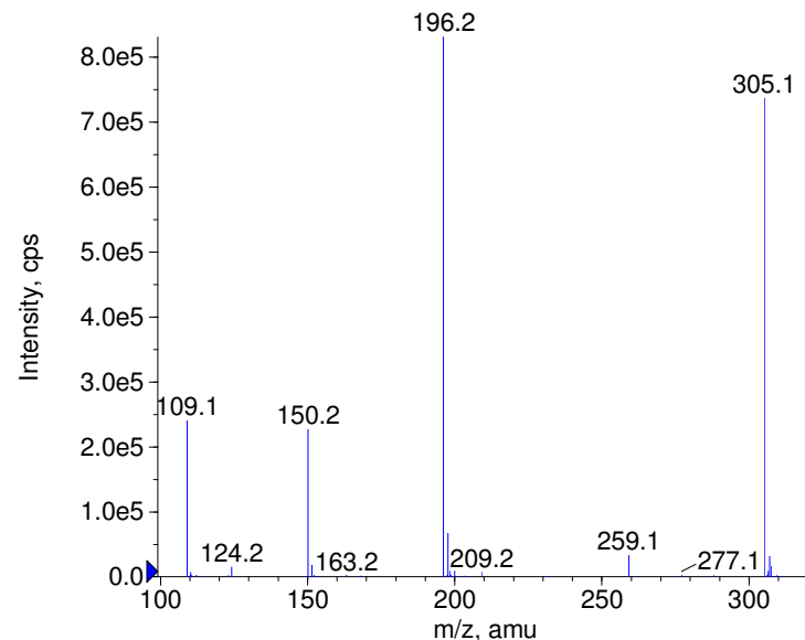
+ Flupirtine Prec(305.0) CE(50.0) RT(0.8)
