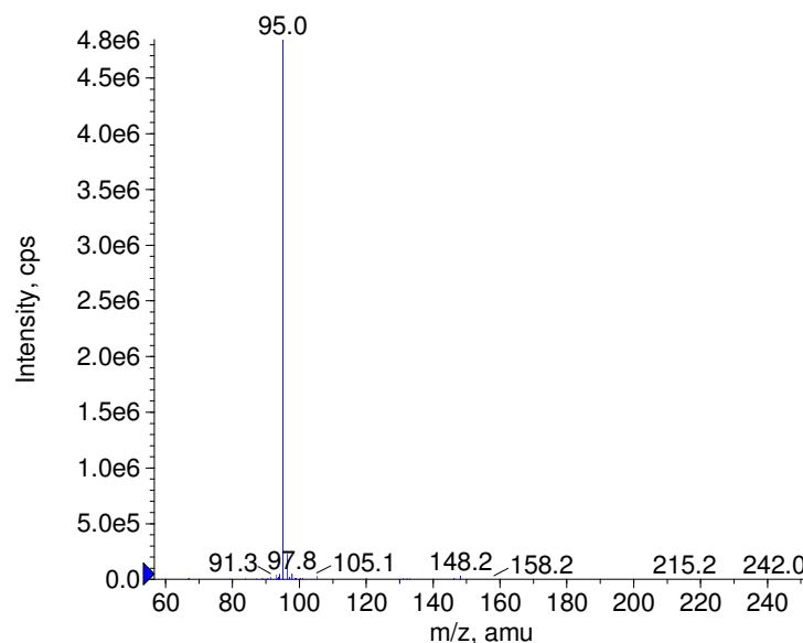
+ Furalaxyl Prec(302.0) CE(50.0) RT(1.2)
