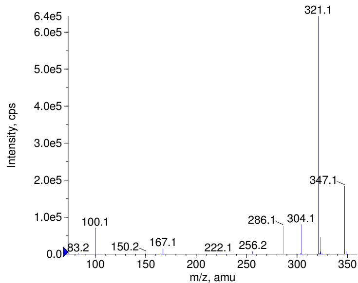
+ Glipizide Prec(446.0) CE(50.0) RT(0.8)
