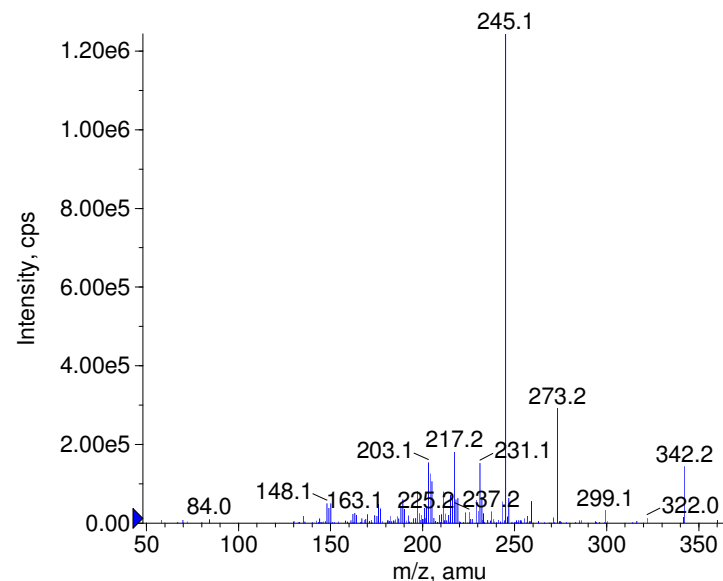
+ Grepafloxacin Prec(360.0) CE(50.0) RT(0.9)
