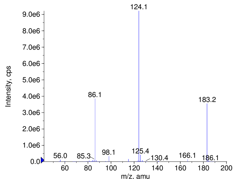
+ Guanacine Prec(183.0) CE(50.0) RT(1.6)
