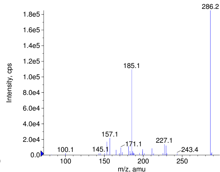
+ Hydromorphone Prec(286.0) CE(99.0) RT(0.9)
