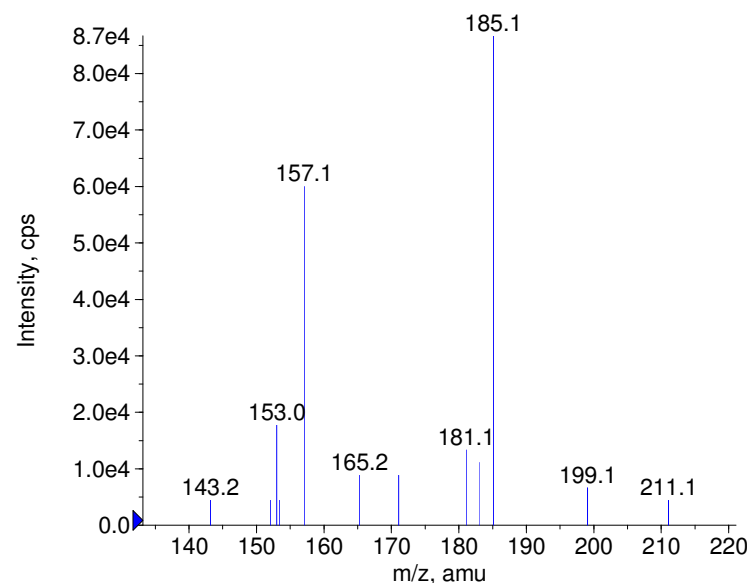
+ Hydromorphone Prec(286.0) CE(50.0) RT(0.9)
