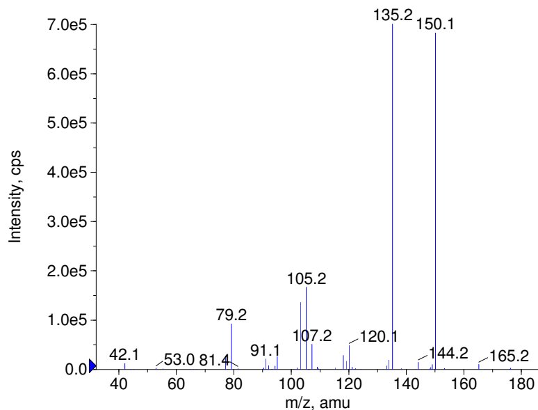
+ 2C-H Prec(182.0) CE(35.0) RT(0.4)
