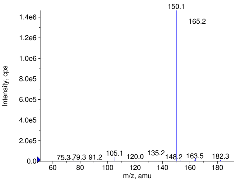
+ 2C-H Prec(182.0) CE(50.0) RT(0.4)
