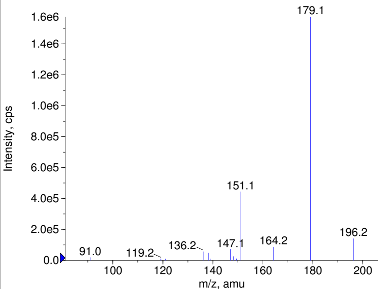
+ 3,4-DMA Prec(196.0) CE(50.0) RT(0.4)
