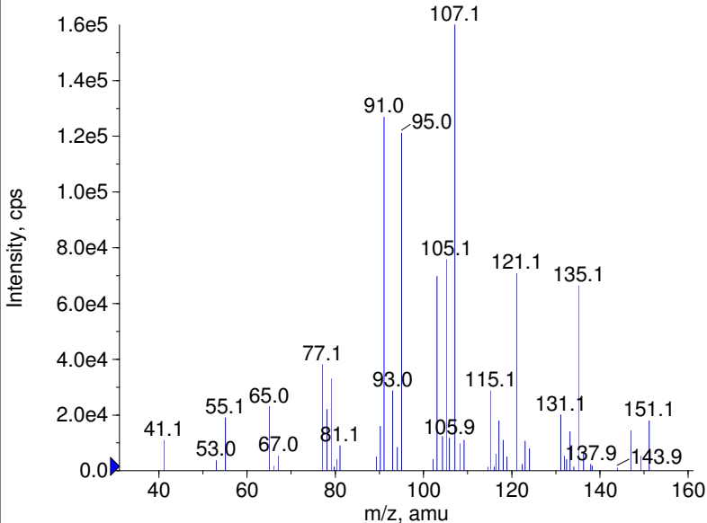
+ 3,4-DMA Prec(196.0) CE(50.0) RT(0.4)
