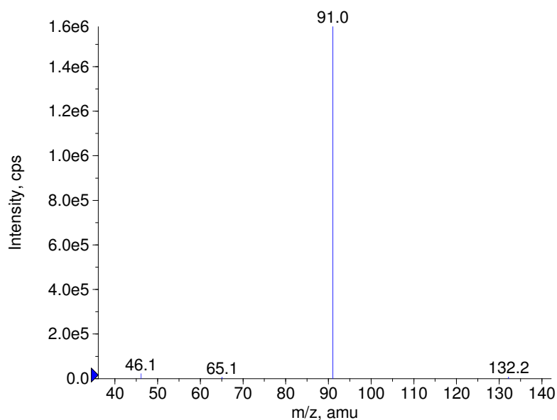
■ + N-Ethyl-amphetamin Prec(164.0) CE(35.0) RT(0.3)
