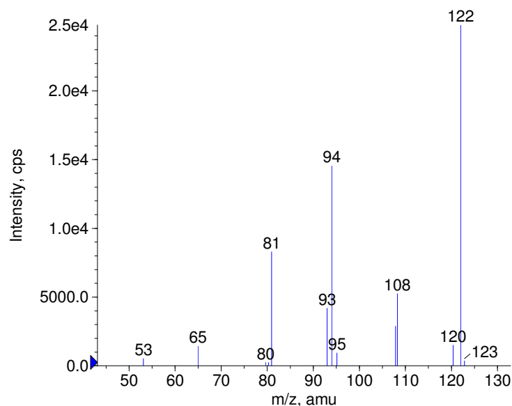
+ 4-(Dimethylamino)phenol Prec(138.0) CE(50.0) RT(1.0)
