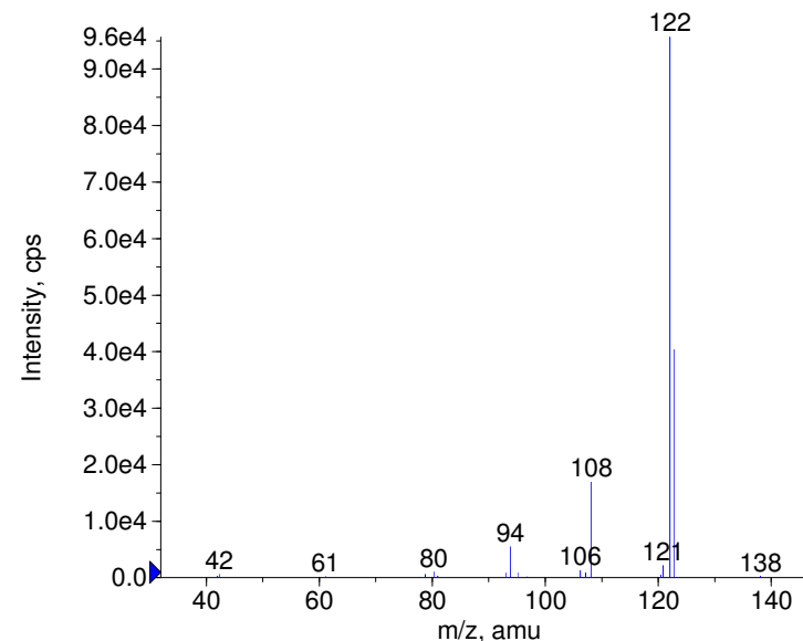
+ 4-(Dimethylamino)phenol Prec(138.0) CE(35.0) RT(1.0)
