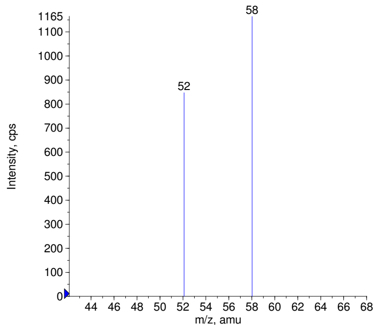
■ + Acipimox Prec(155.0) CE(50.0) RT(0.4)
