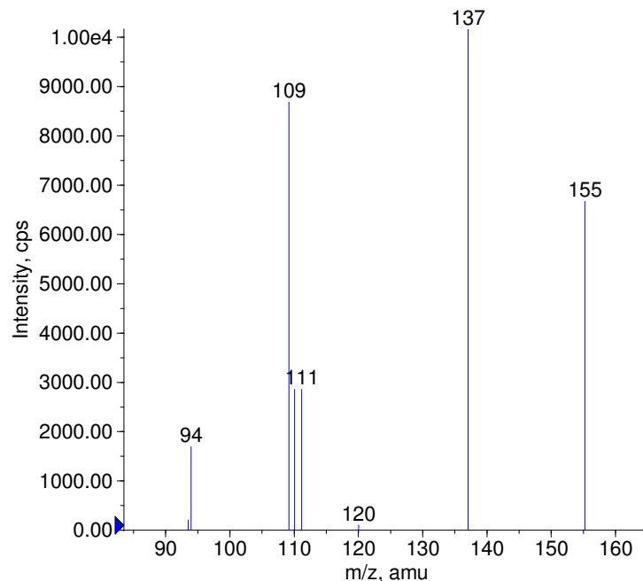
■ + Acipimox Prec(155.0) CE(50.0) RT(0.4)
