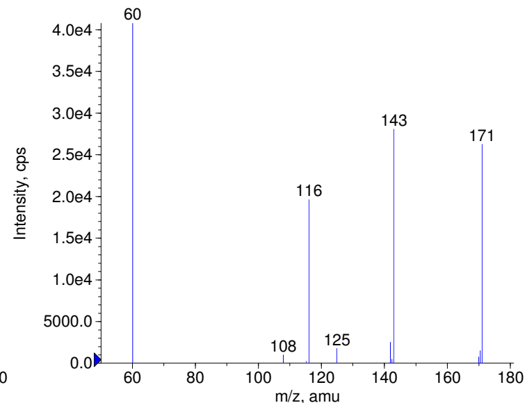
+ Amiloride Prec(230.0) CE(35.0) RT(0.2)
