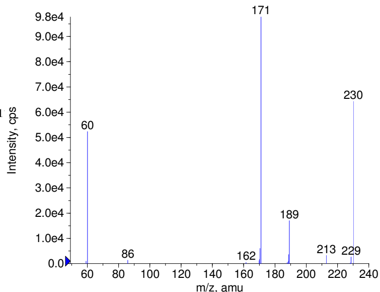
+ Amiloride Prec(230.0) CE(50.0) RT(0.3)
