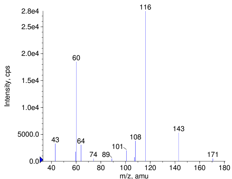
+ Amiloride Prec(230.0) CE(50.0) RT(0.3)
