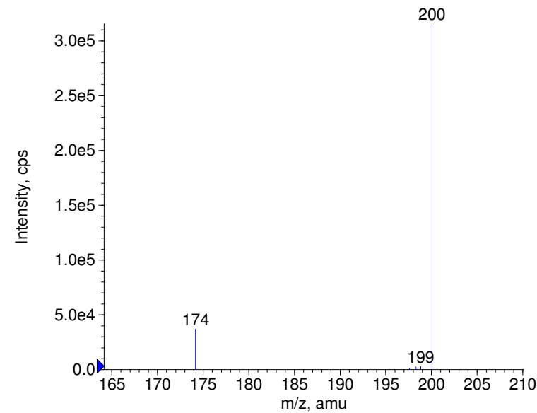
■ + Aminoquinuride Prec(373.0) CE(35.0) RT(0.2)
