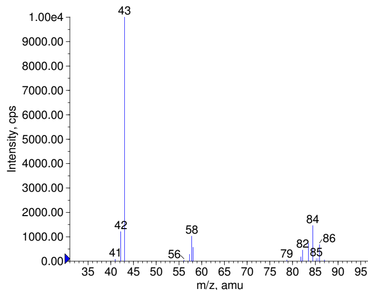
■ + Amitrole Prec(85.0) CE(50.0) RT(0.3)
