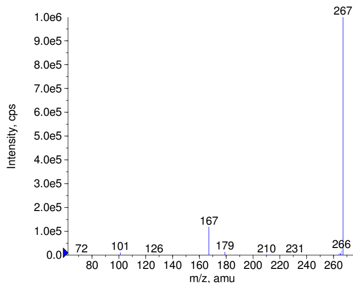
+ Anilazine Prec(267.0) CE(50.0) RT(0.3)
