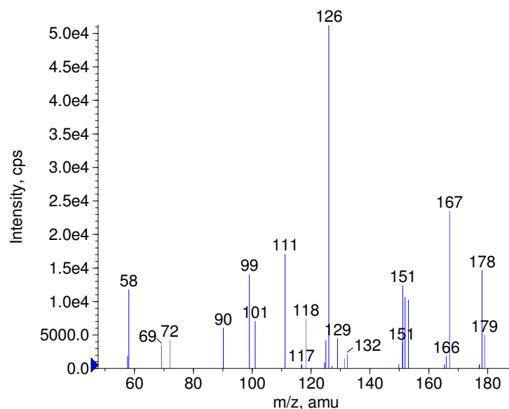
+ Anilazine Prec(267.0) CE(50.0) RT(0.3)
