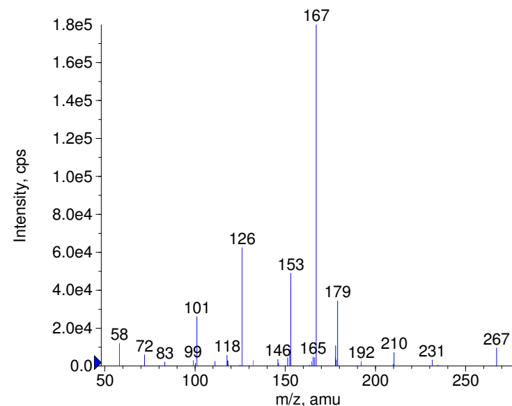
+ Anilazine Prec(267.0) CE(35.0) RT(0.2)
