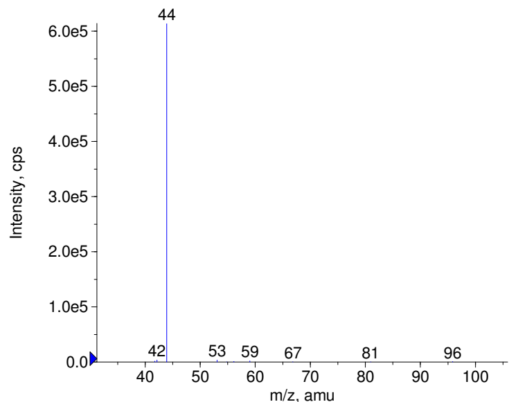
+ Arecoline Prec(156.0) CE(50.0) RT(1.3)
