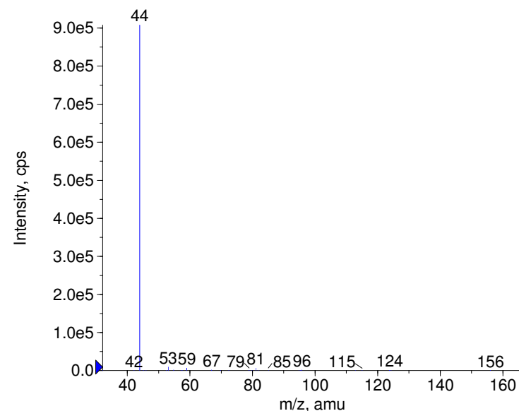
+ Arecoline Prec(156.0) CE(35.0) RT(1.3)
