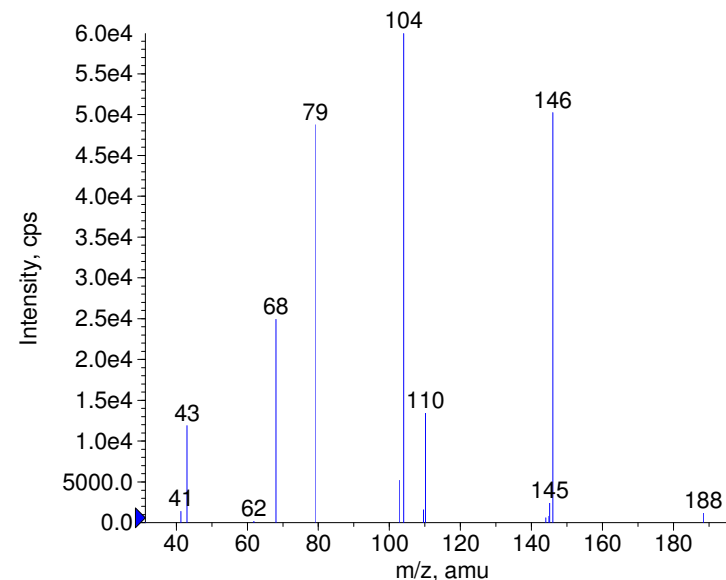
+ Atrazine-desethyl Prec(188.0) CE(35.0) RT(0.2)
