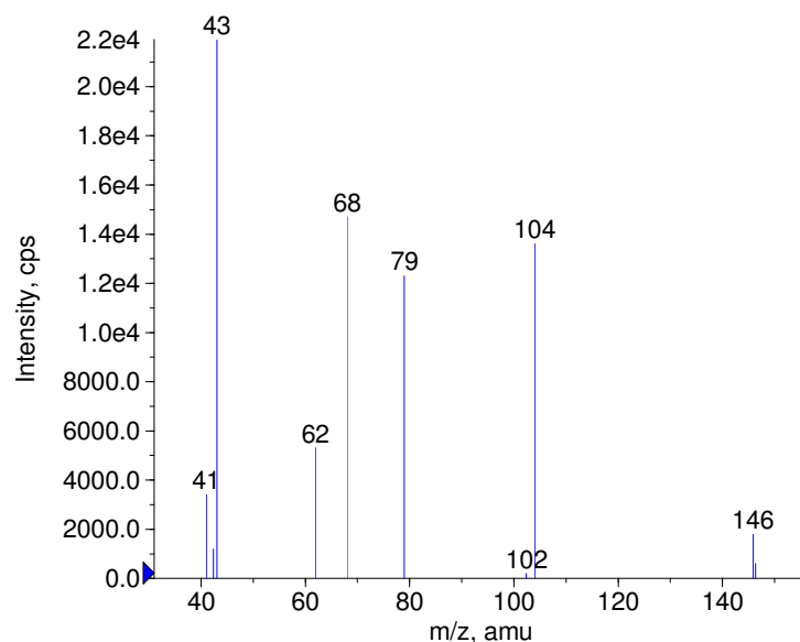
+ Atrazine-desethyl Prec(188.0) CE(50.0) RT(0.3)
