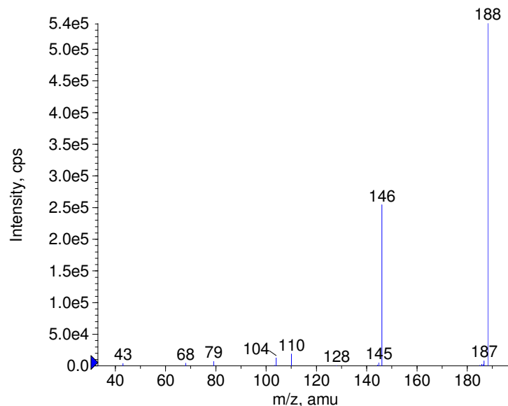
+ Atrazine-desethyl Prec(188.0) CE(50.0) RT(0.3)
