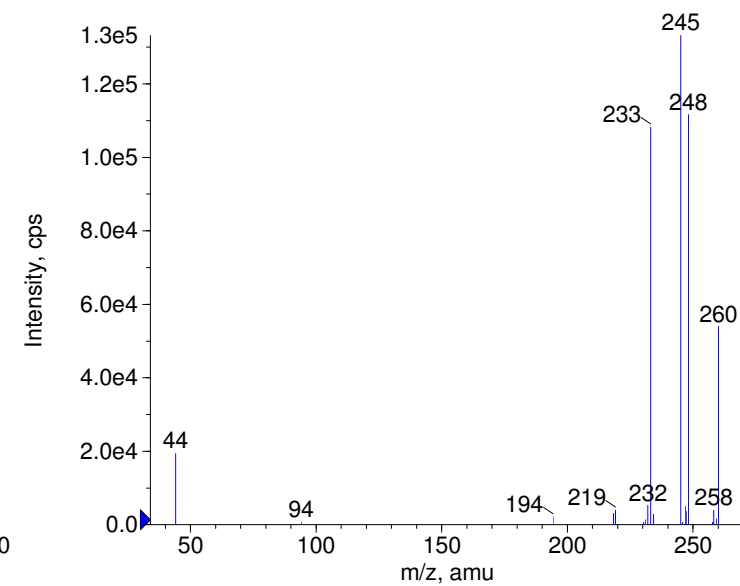
+ Azatadine Prec(291.0) CE(35.0) RT(0.2)
