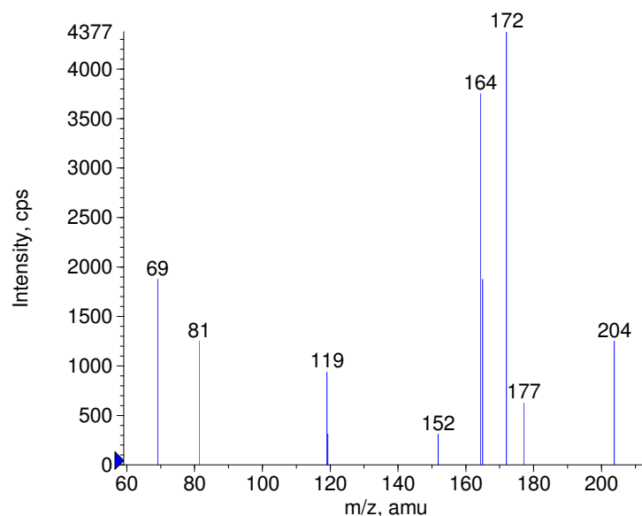
+ Azathioprine Prec(278.0) CE(50.0) RT(0.3)
