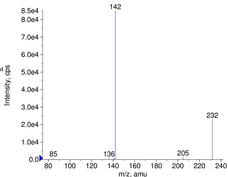
+ Azathioprine Prec(278.0) CE(50.0) RT(0.3)
