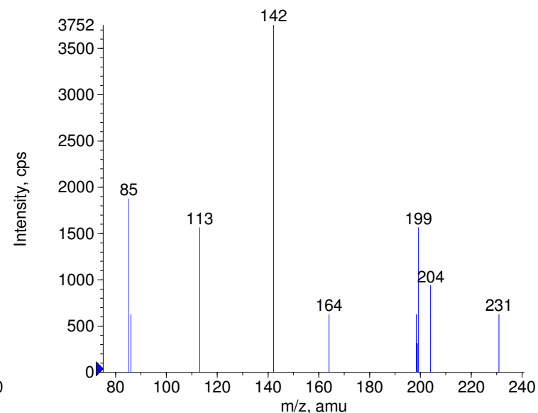
+ Azathioprine Prec(278.0) CE(35.0) RT(0.2)
