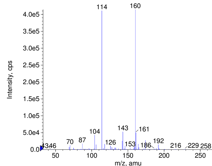
+ Azidocillin Prec(376.0) CE(35.0) RT(3.5)
