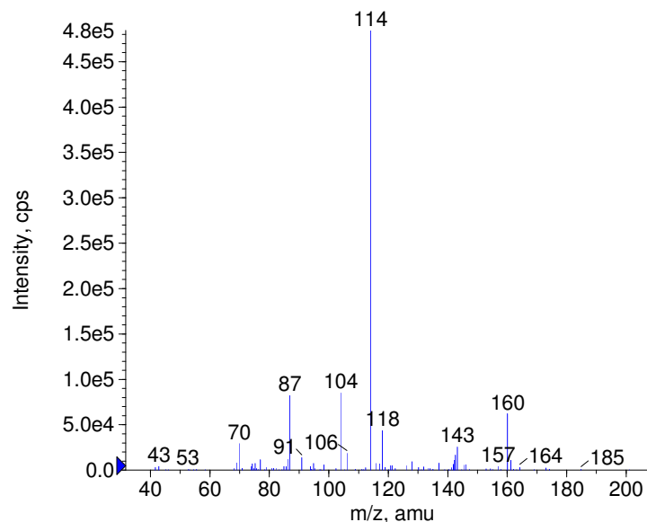
+ Azidocillin Prec(376.0) CE(50.0) RT(3.5)
