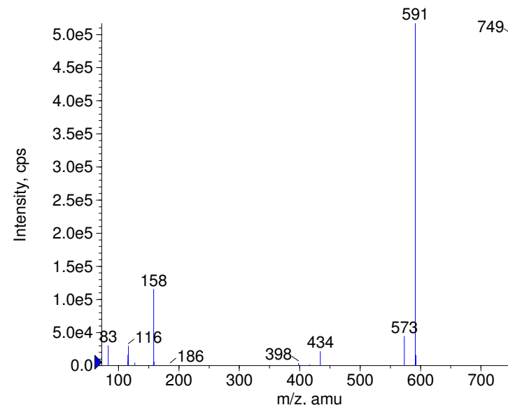
+ Azithromycin Prec(749.5) CE(35.0) RT(2.2)
