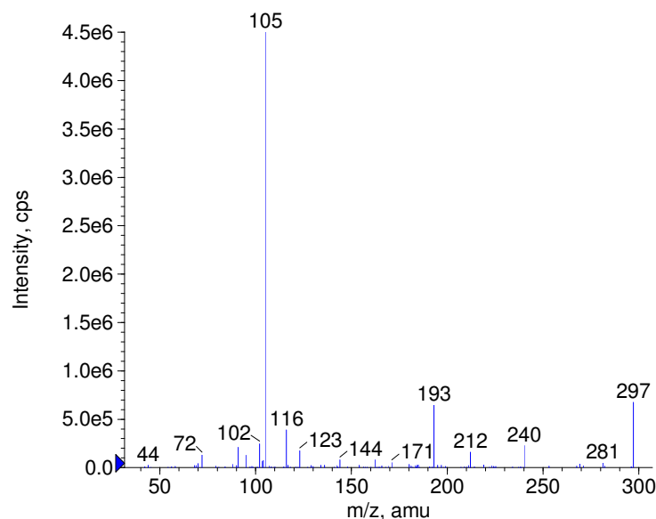
+ Bamifylline Prec(386.0) CE(50.0) RT(2.3)
