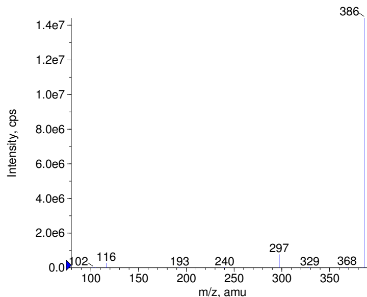
+ Bamifylline Prec(386.0) CE(50.0) RT(2.3)
