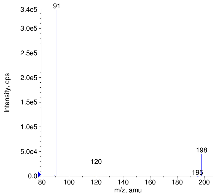
+ Beclamide Prec(198.0) CE(50.0) RT(0.5)
