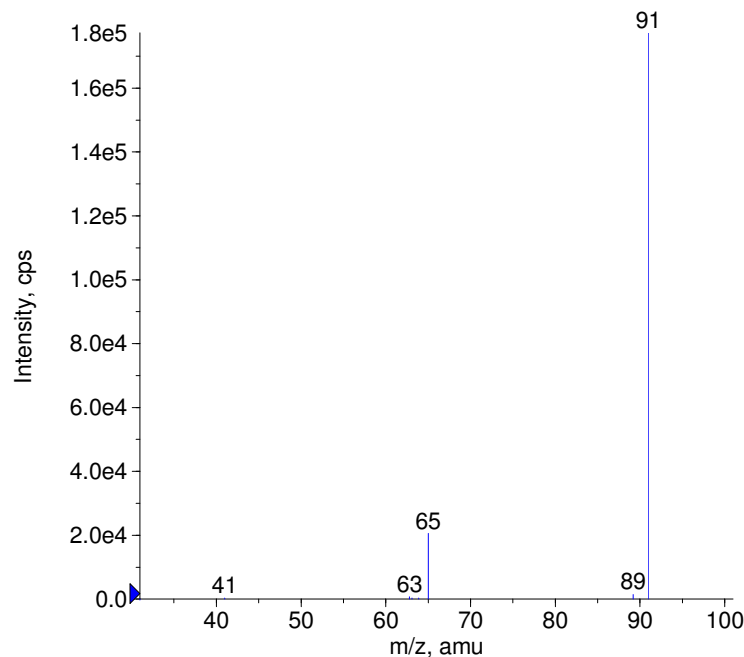
+ Beclamide Prec(198.0) CE(50.0) RT(0.5)
